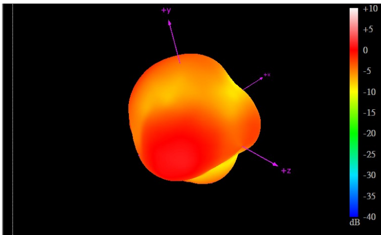
1575.42MHz
